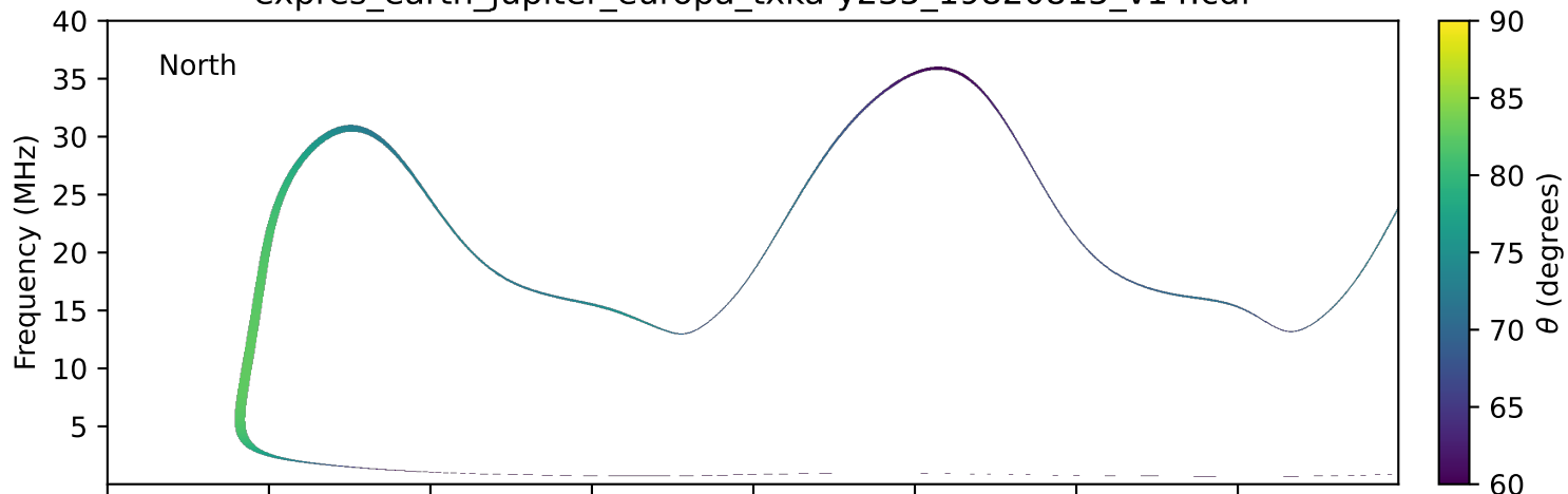
expres_earth_jupiter_europa_txka-y235_19820815_v14.cdf
