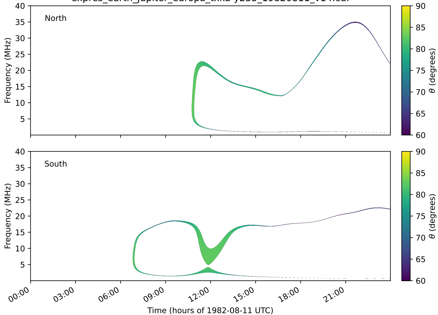
expres_earth_jupiter_europa_txka-y235_19820811_v14.cdf
