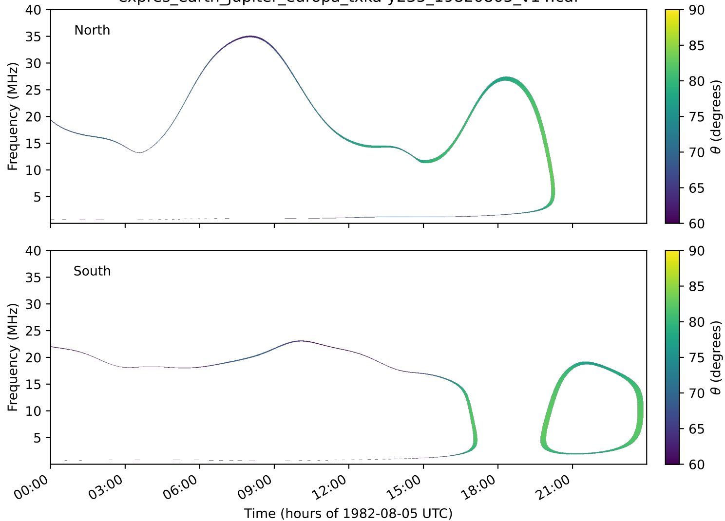
expres_earth_jupiter_europa_txka-y235_19820805_v14.cdf
