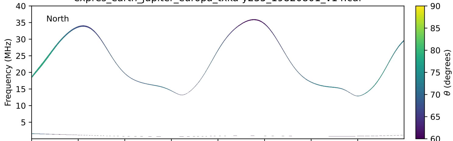
expres_earth_jupiter_europa_txka-y235_19820801_v14.cdf
