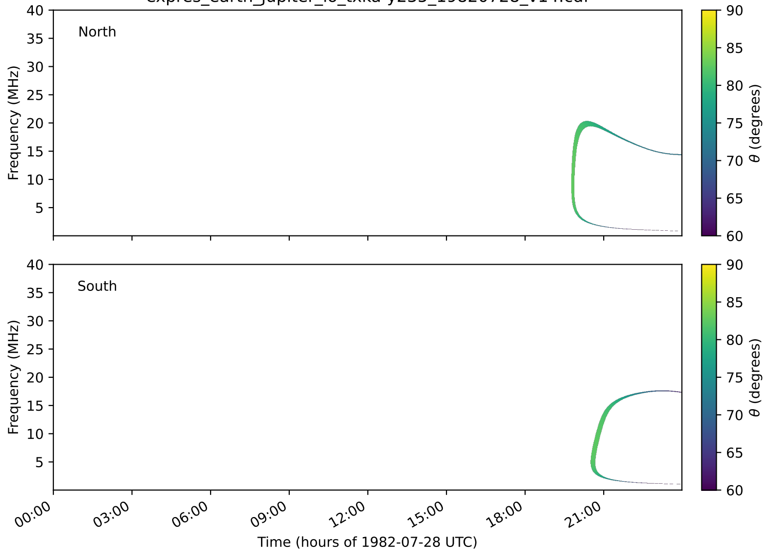
expres_earth_jupiter_io_txka-y235_19820728_v14.cdf
