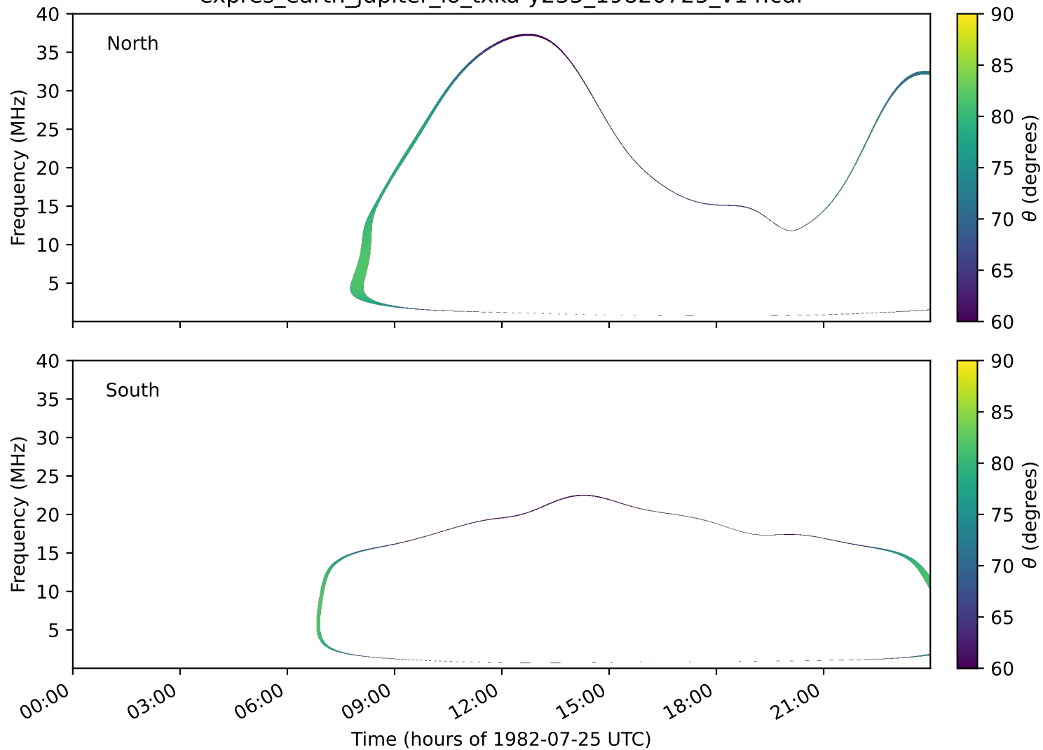
expres_earth_jupiter_io_txka-y235_19820725_v14.cdf
