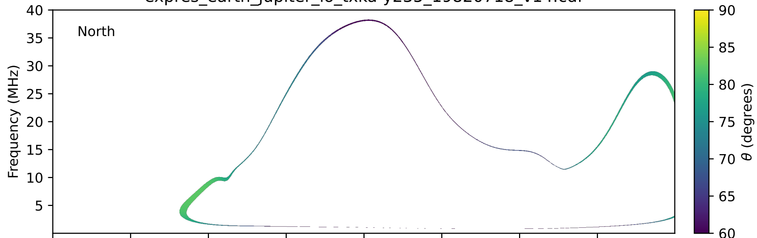
expres_earth_jupiter_io_txka-y235_19820718_v14.cdf
