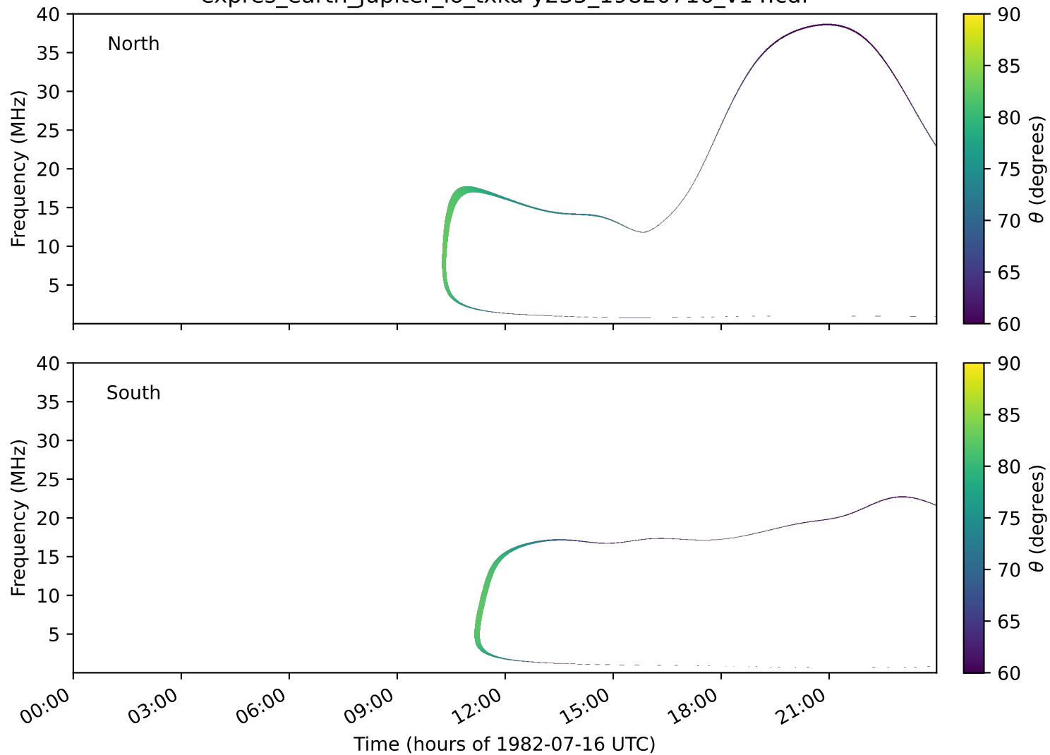
expres_earth_jupiter_io_txka-y235_19820716_v14.cdf
