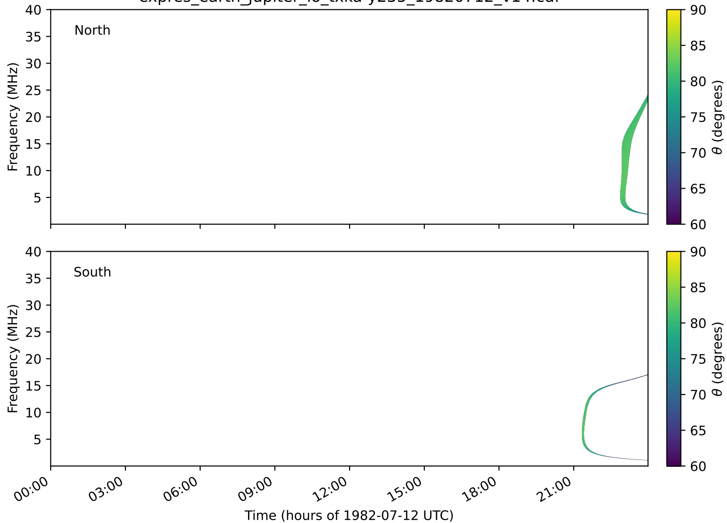
expres_earth_jupiter_io_txka-y235_19820712_v14.cdf
