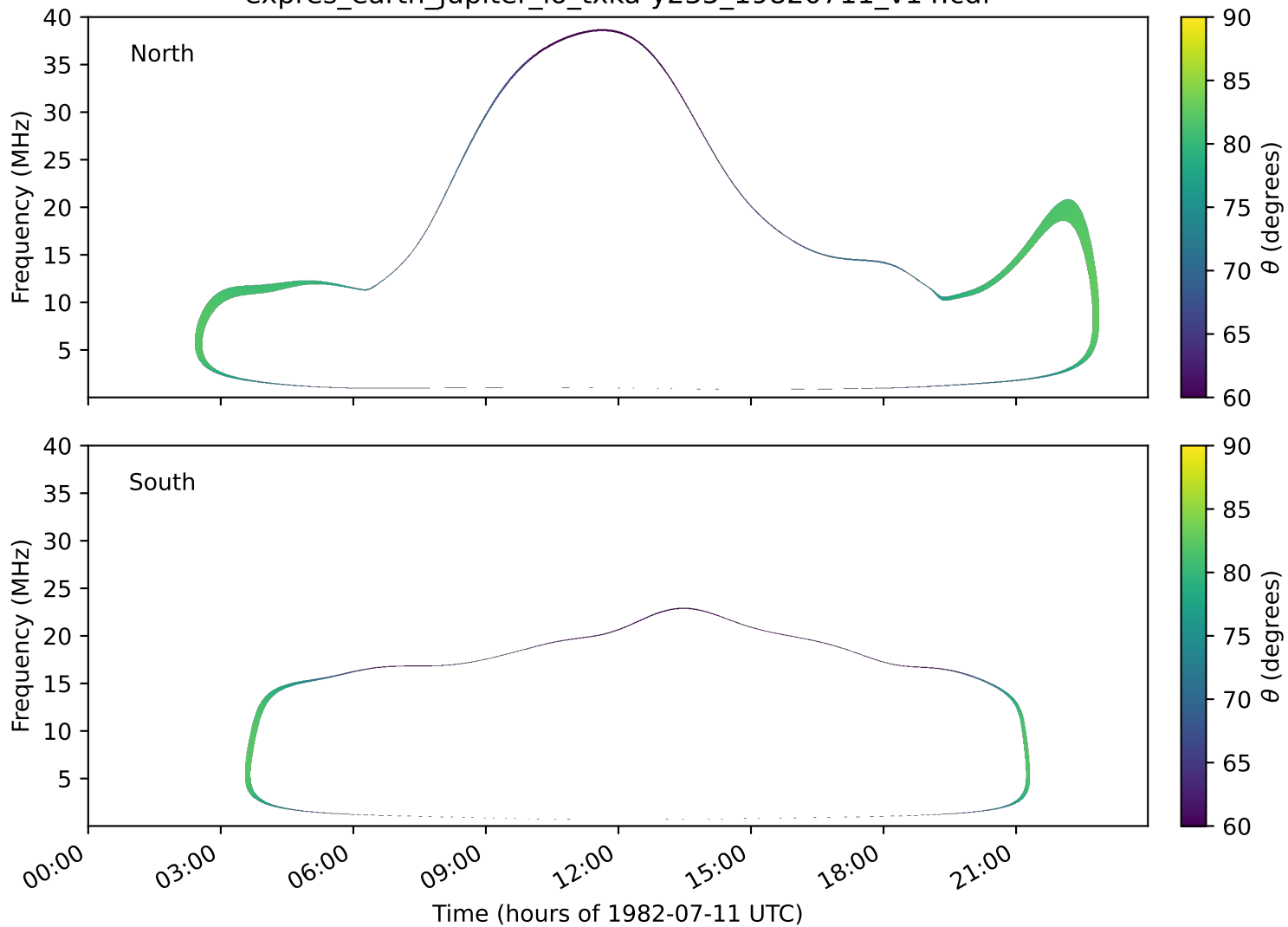
expres_earth_jupiter_io_txka-y235_19820711_v14.cdf
