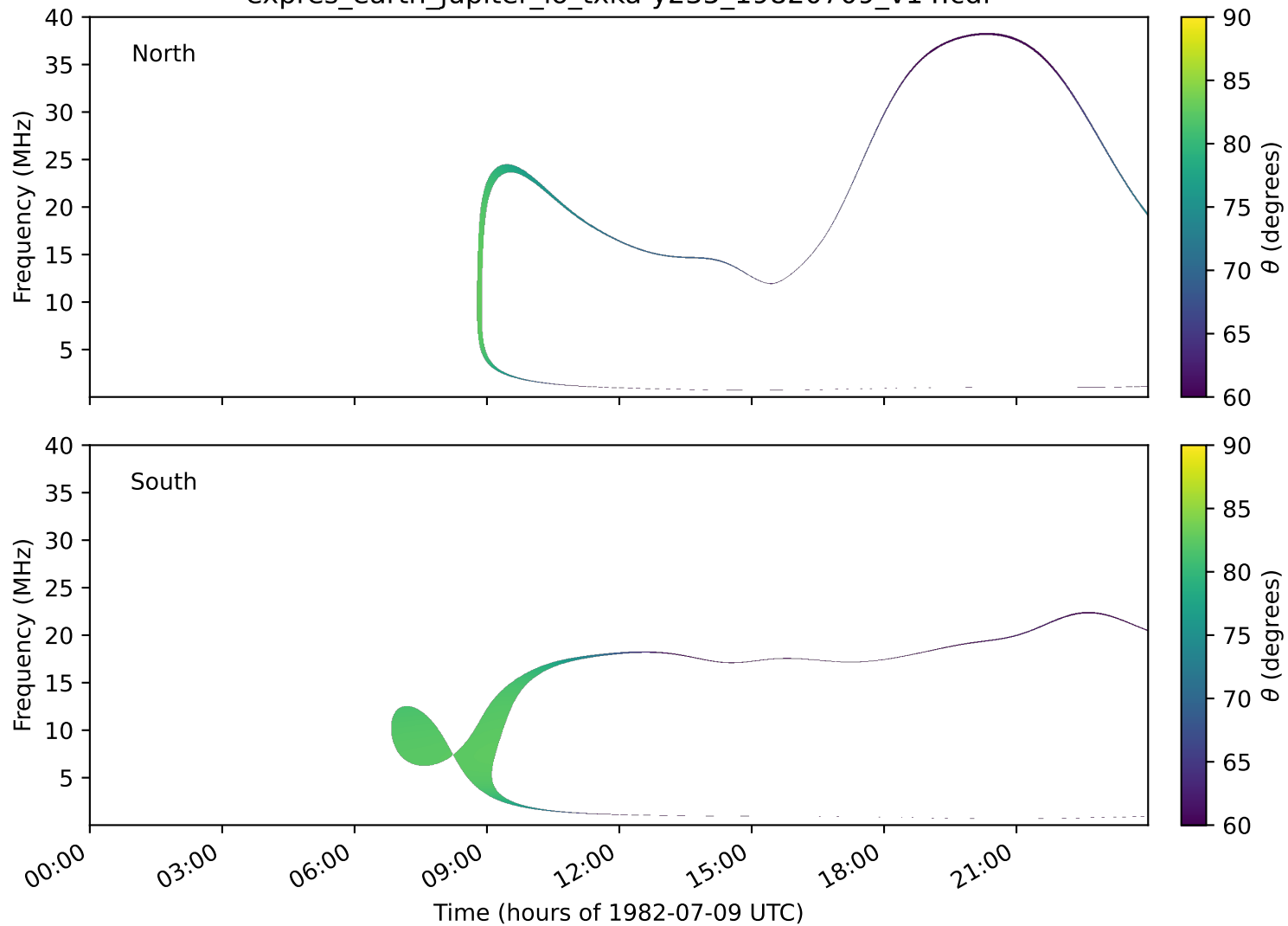
expres_earth_jupiter_io_txka-y235_19820709_v14.cdf
