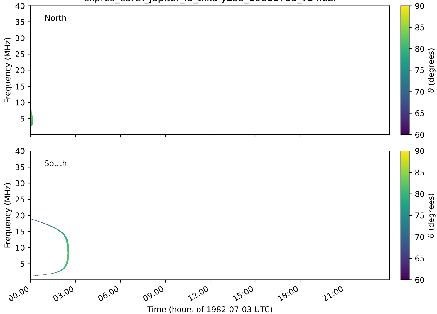
expres_earth_jupiter_io_txka-y235_19820703_v14.cdf
