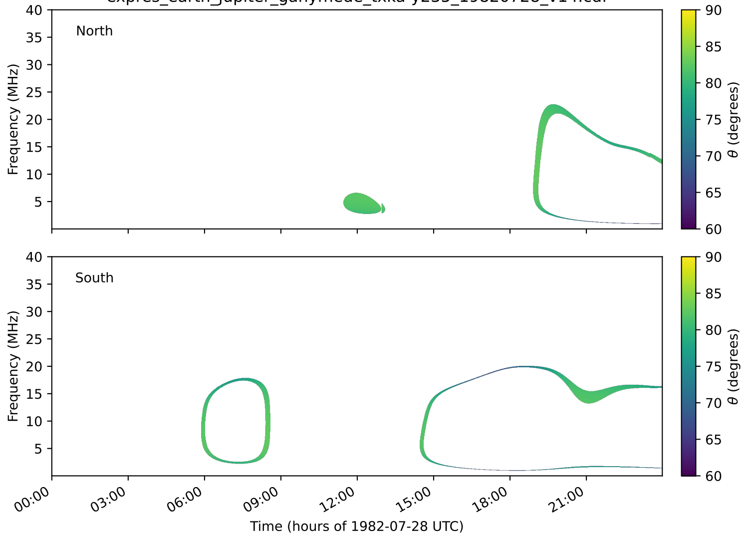
expres_earth_jupiter_ganymede_txka-y235_19820728_v14.cdf
