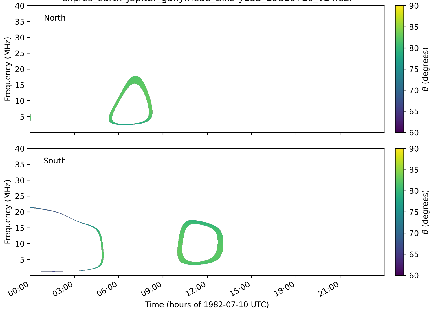
expres_earth_jupiter_ganymede_txka-y235_19820710_v14.cdf
