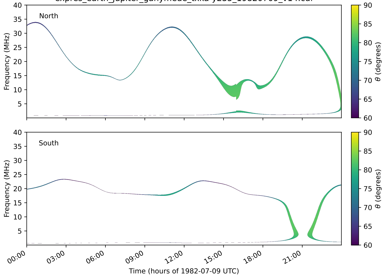
expres_earth_jupiter_ganymede_txka-y235_19820709_v14.cdf
