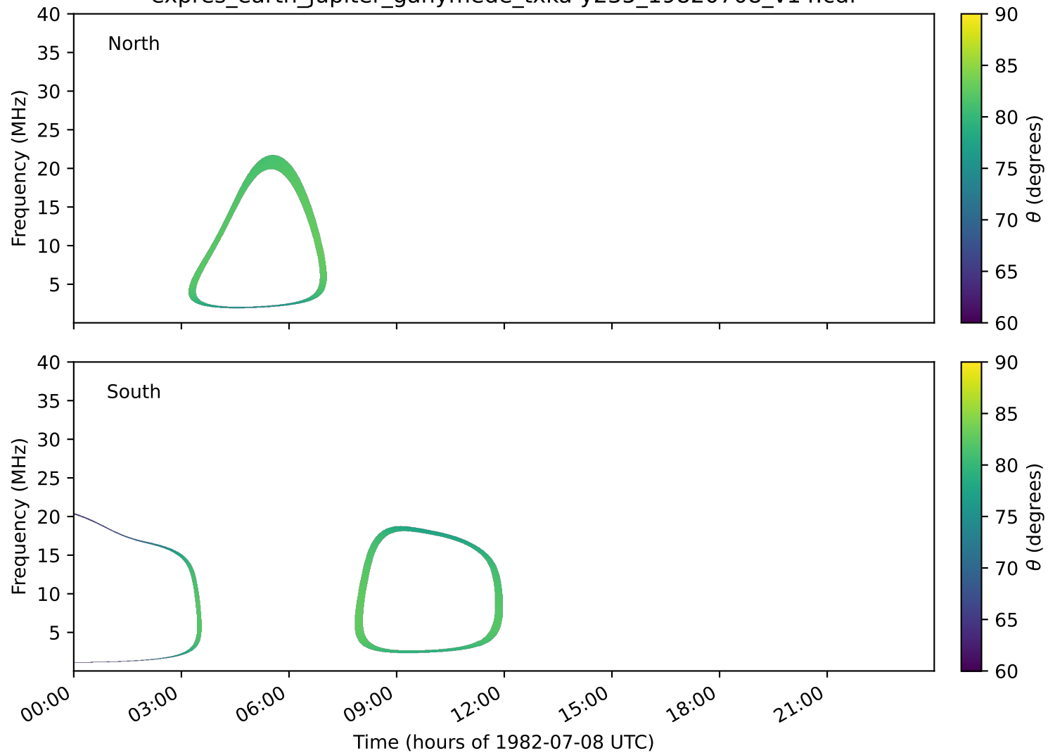
expres_earth_jupiter_ganymede_txka-y235_19820708_v14.cdf
