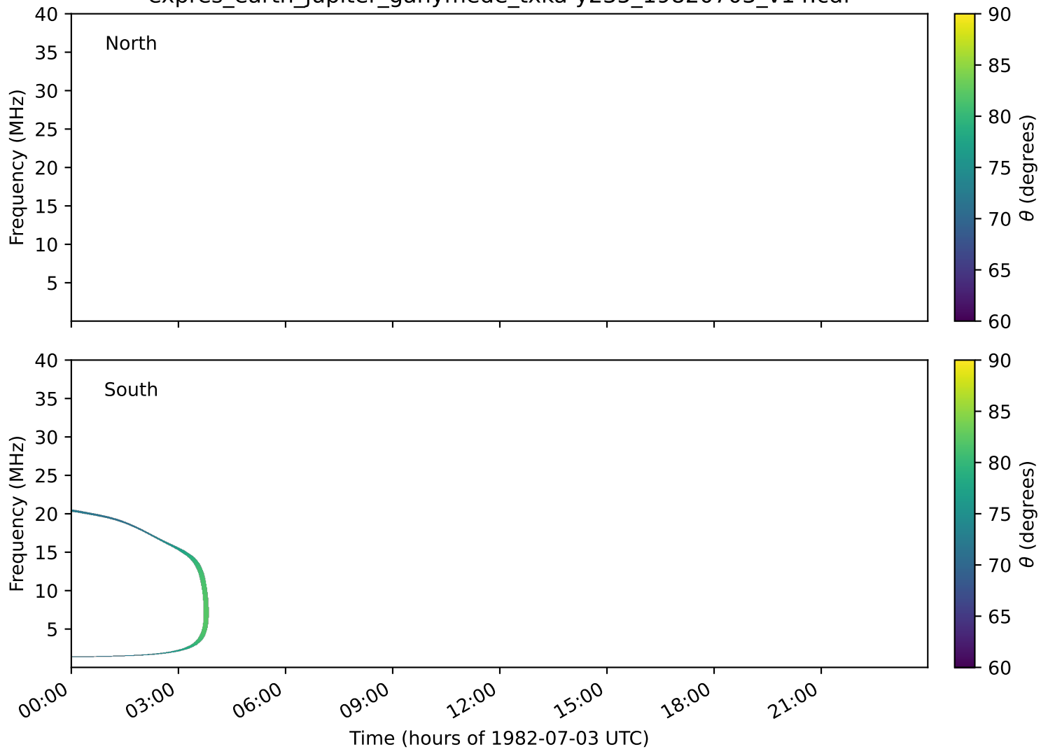
expres_earth_jupiter_ganymede_txka-y235_19820703_v14.cdf
