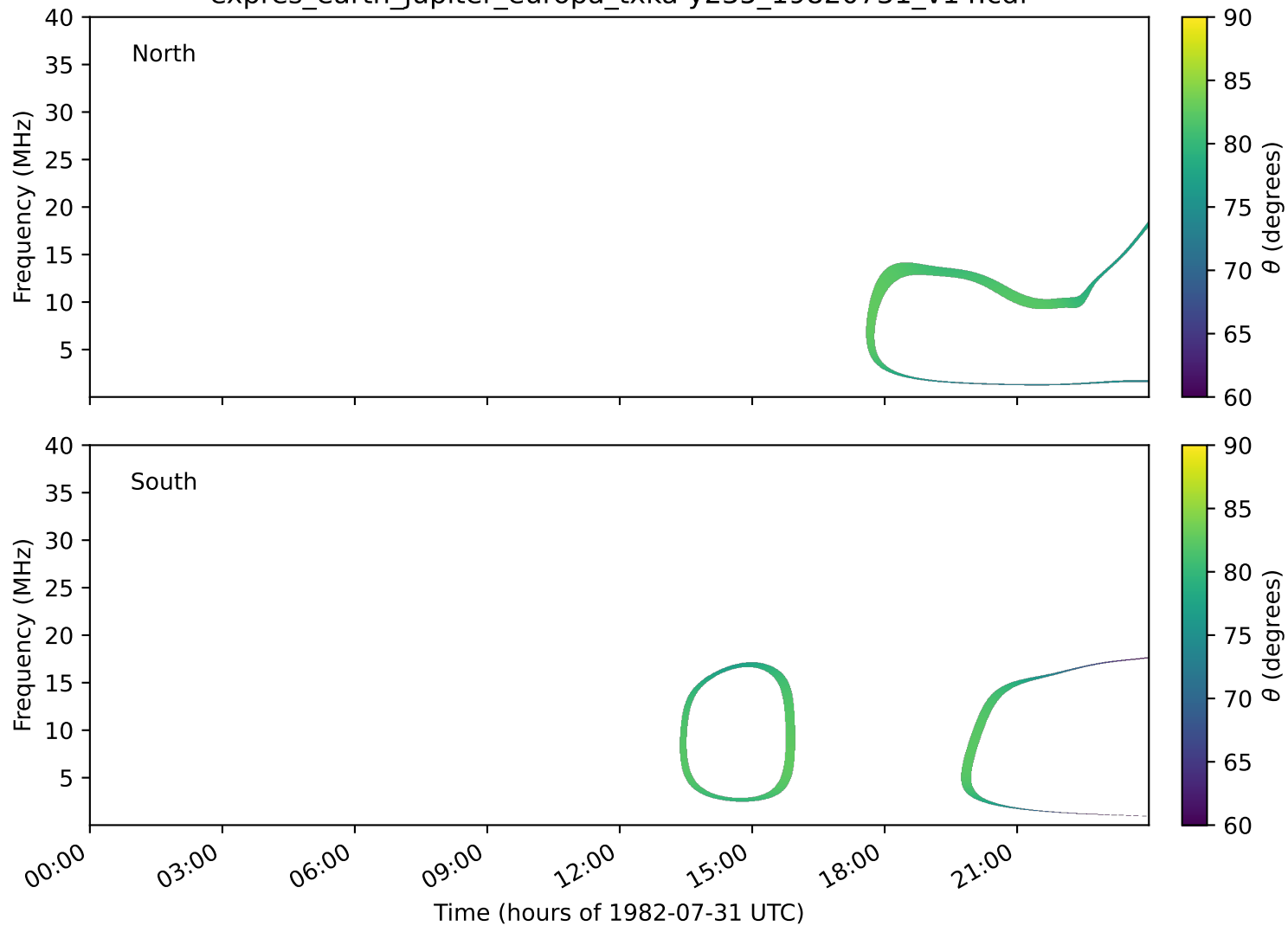
expres_earth_jupiter_europa_txka-y235_19820731_v14.cdf
