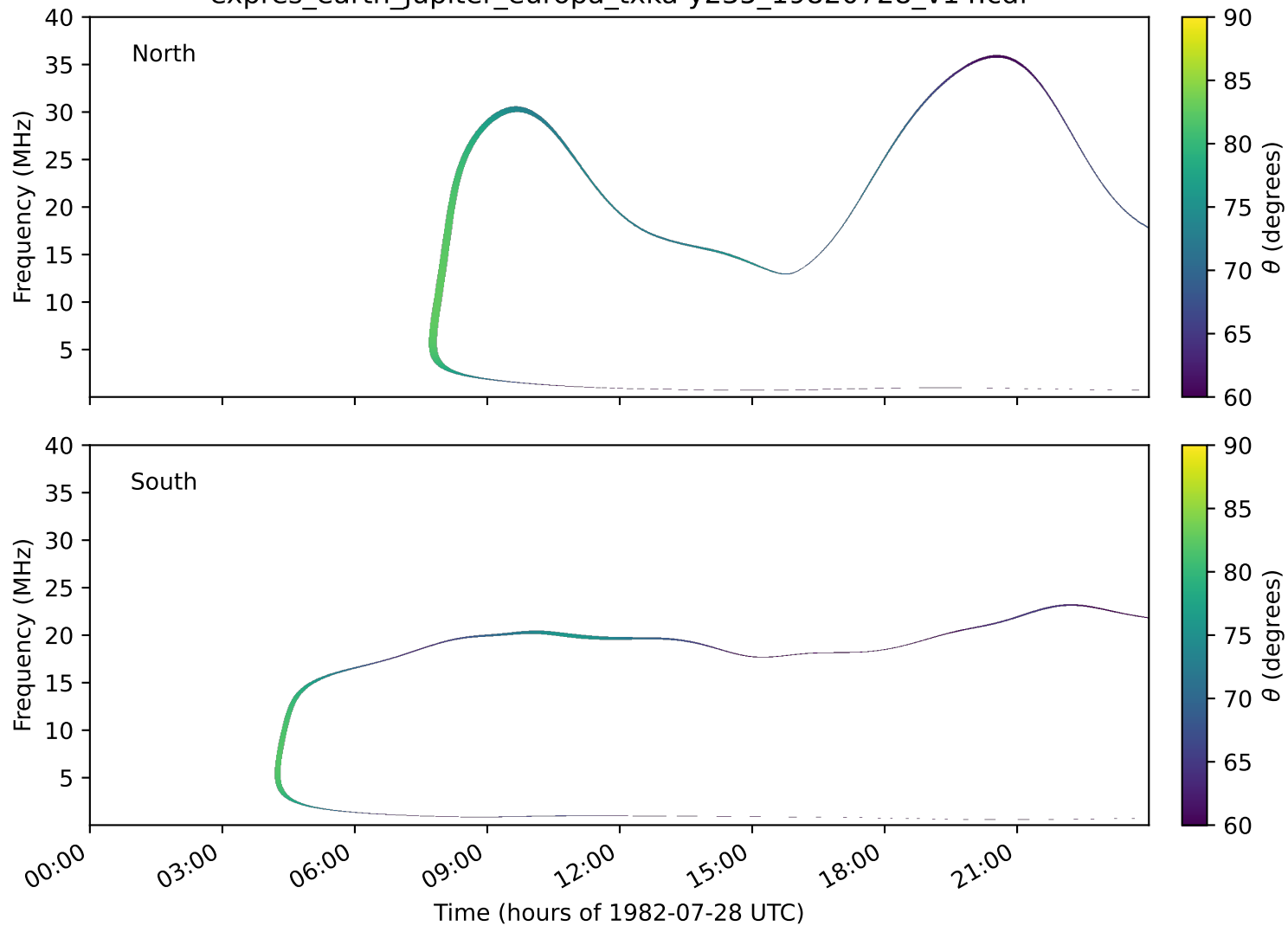
expres_earth_jupiter_europa_txka-y235_19820728_v14.cdf
