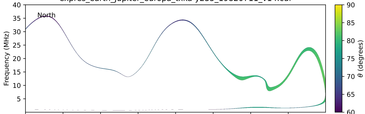
expres_earth_jupiter_europa_txka-y235_19820711_v14.cdf
