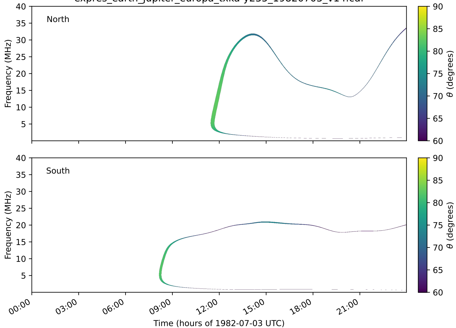
expres_earth_jupiter_europa_txka-y235_19820703_v14.cdf
