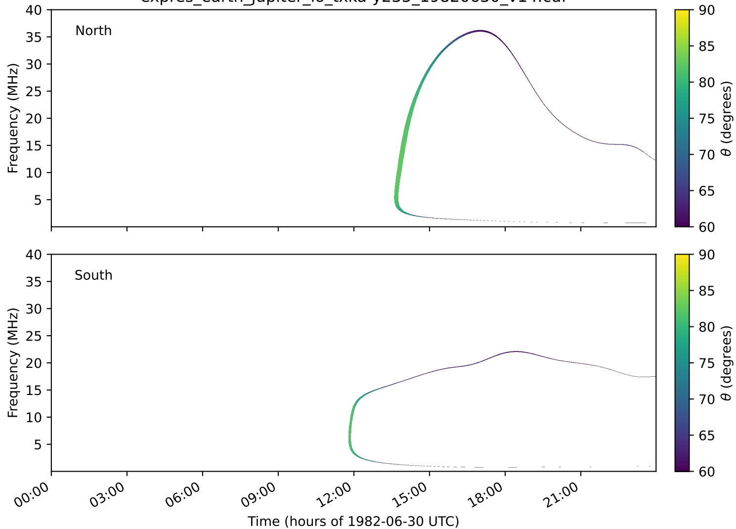
expres_earth_jupiter_io_txka-y235_19820630_v14.cdf
