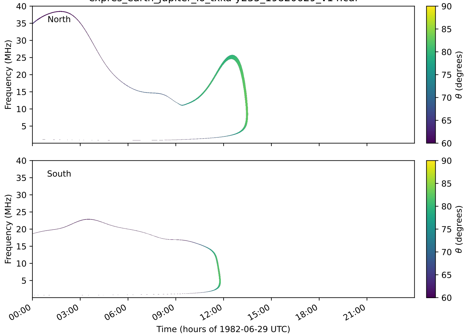
expres_earth_jupiter_io_txka-y235_19820629_v14.cdf
