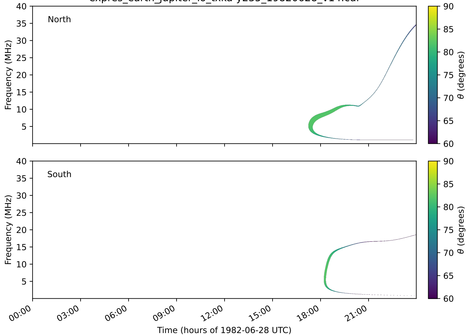
expres_earth_jupiter_io_txka-y235_19820628_v14.cdf
