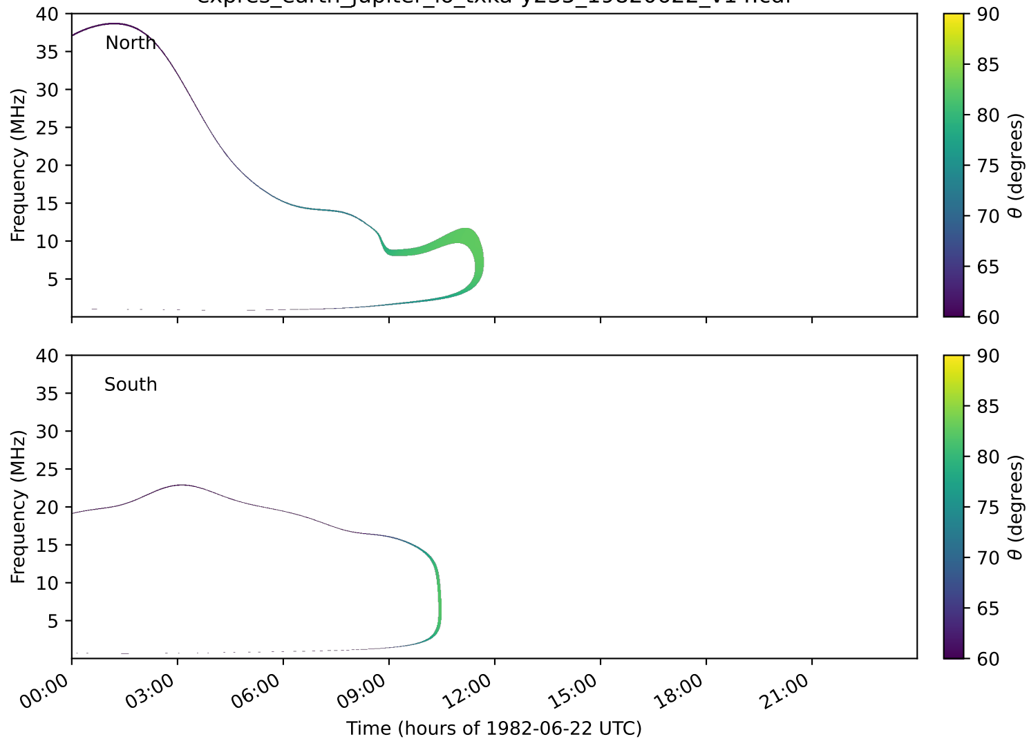
expres_earth_jupiter_io_txka-y235_19820622_v14.cdf
