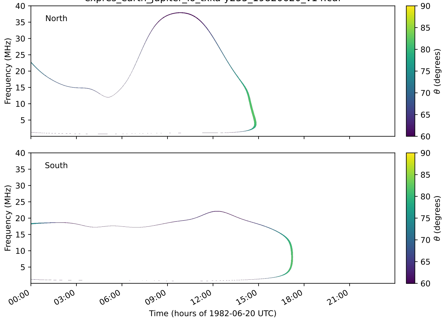
expres_earth_jupiter_io_txka-y235_19820620_v14.cdf
