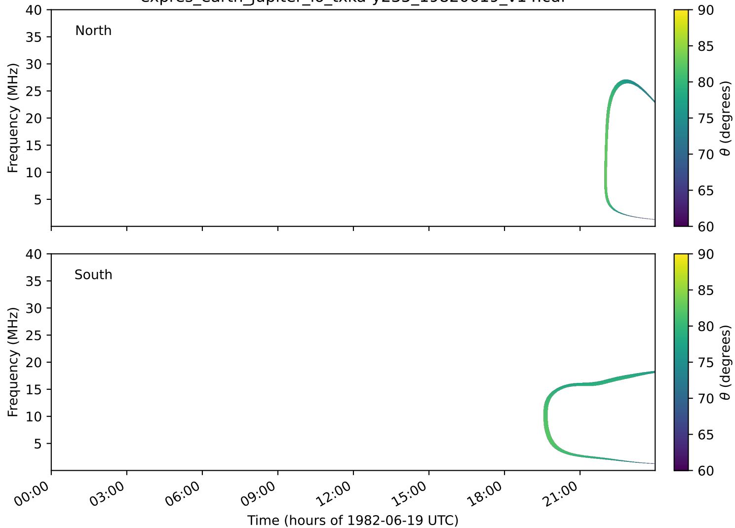
expres_earth_jupiter_io_txka-y235_19820619_v14.cdf
