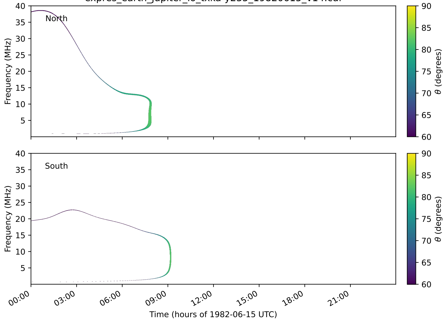
expres_earth_jupiter_io_txka-y235_19820615_v14.cdf
