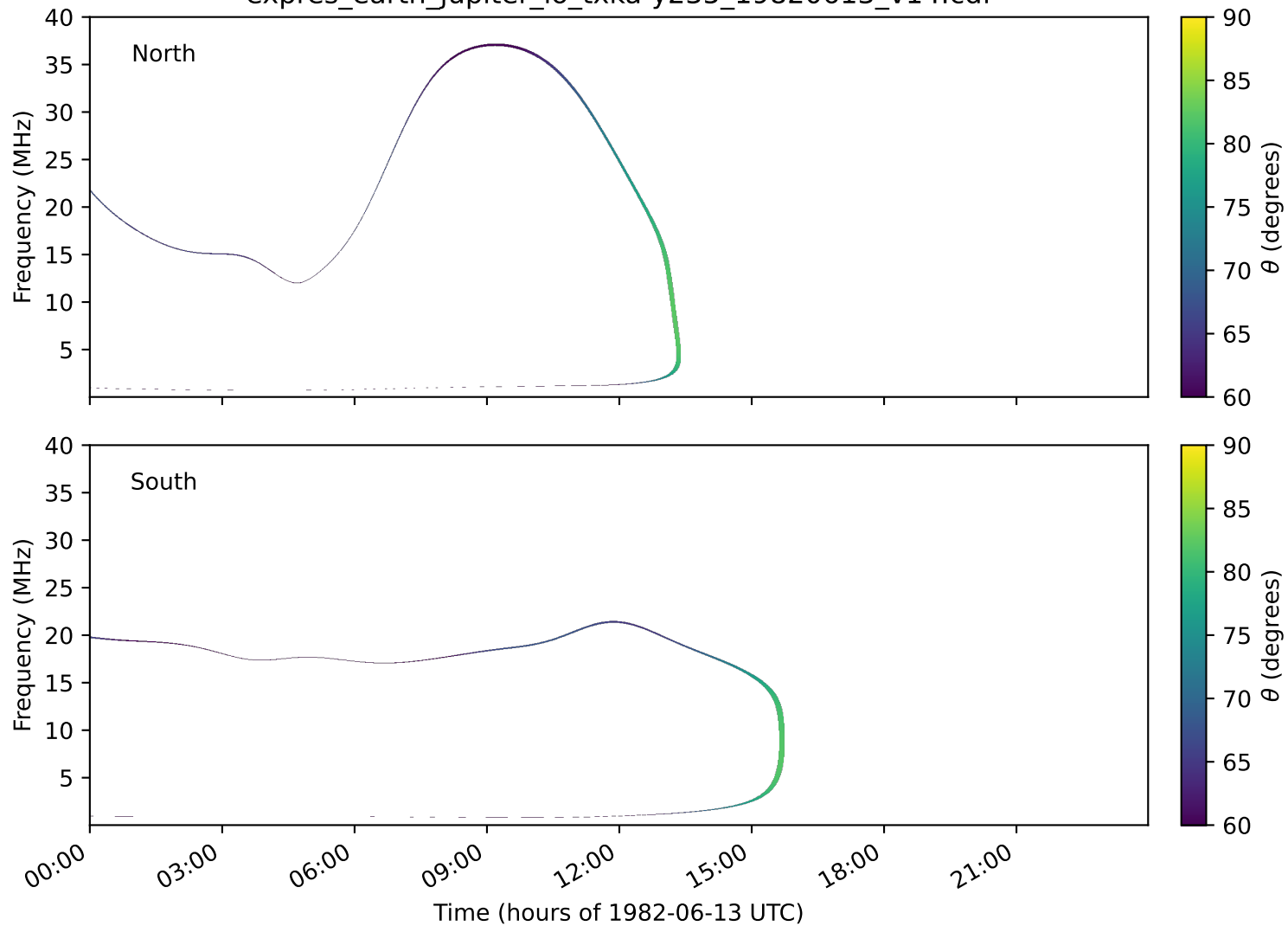
expres_earth_jupiter_io_txka-y235_19820613_v14.cdf
