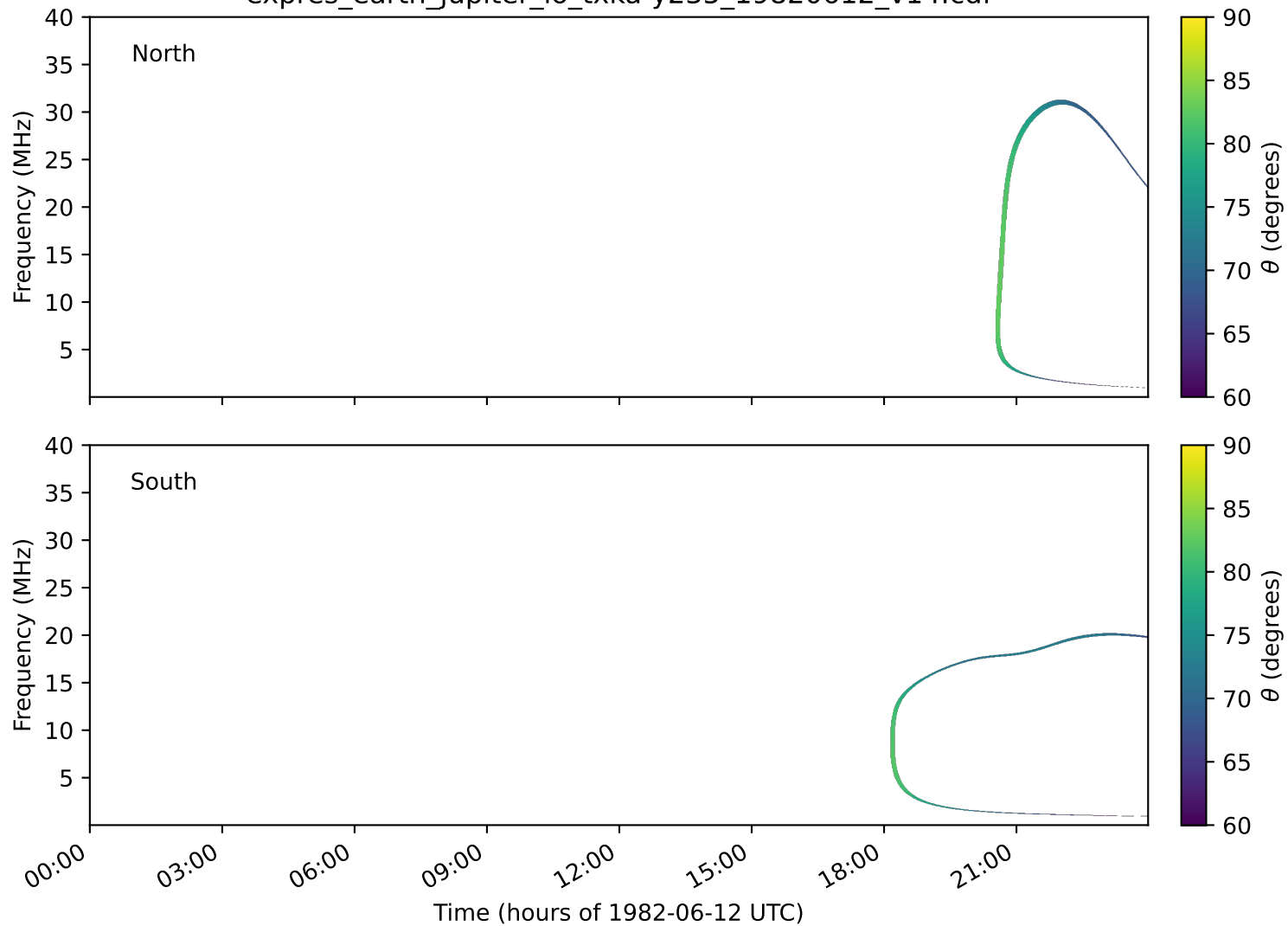
expres_earth_jupiter_io_txka-y235_19820612_v14.cdf
