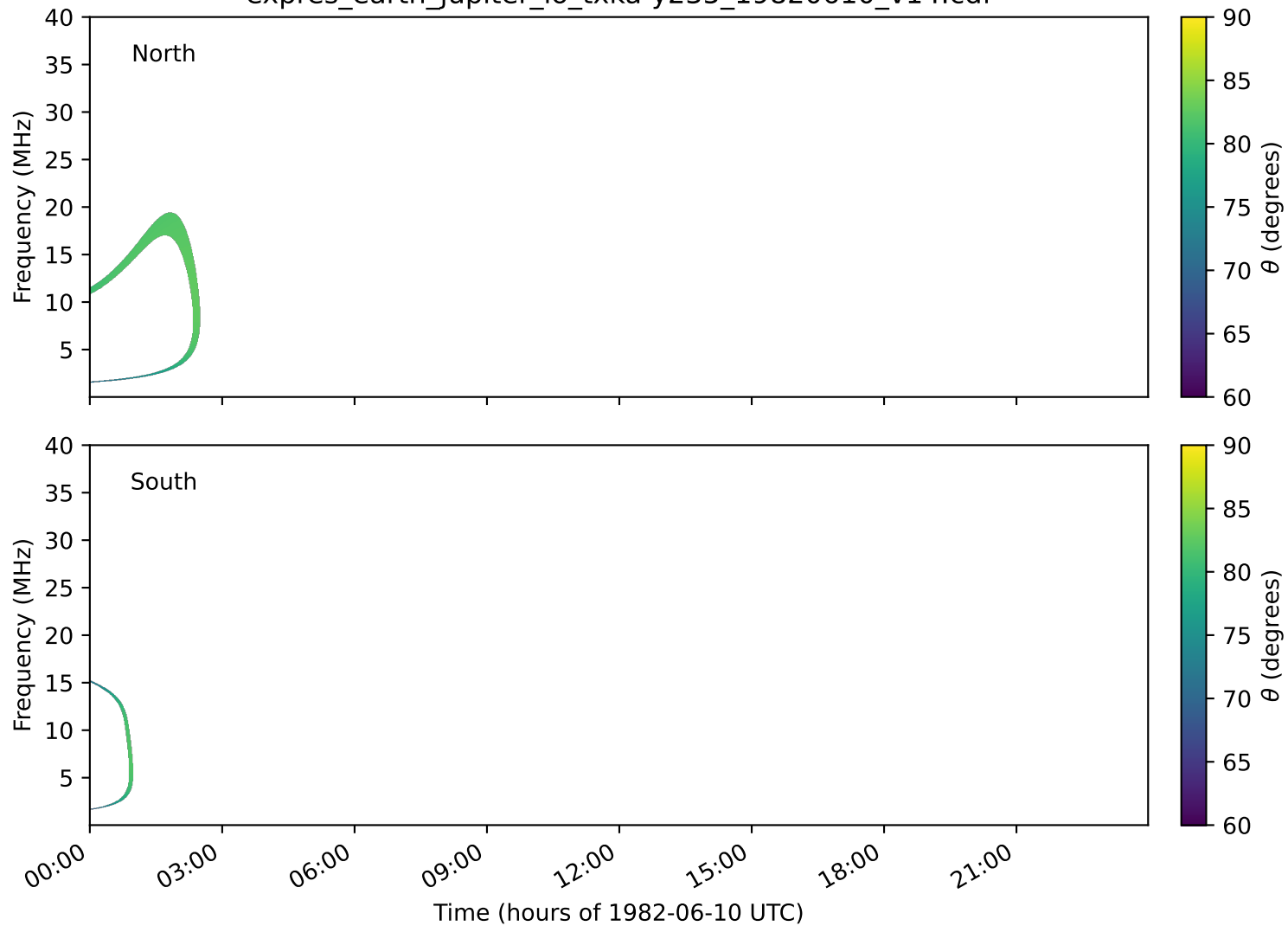
expres_earth_jupiter_io_txka-y235_19820610_v14.cdf
