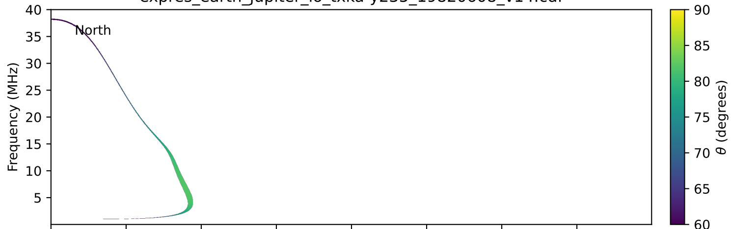
expres_earth_jupiter_io_txka-y235_19820608_v14.cdf
