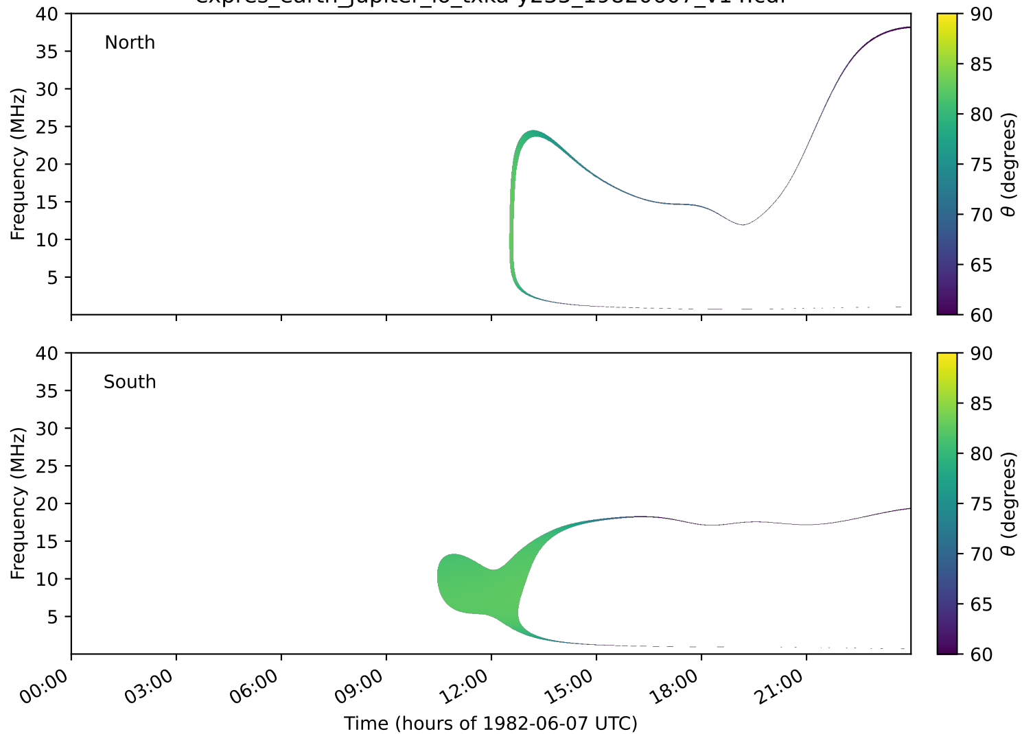
expres_earth_jupiter_io_txka-y235_19820607_v14.cdf
