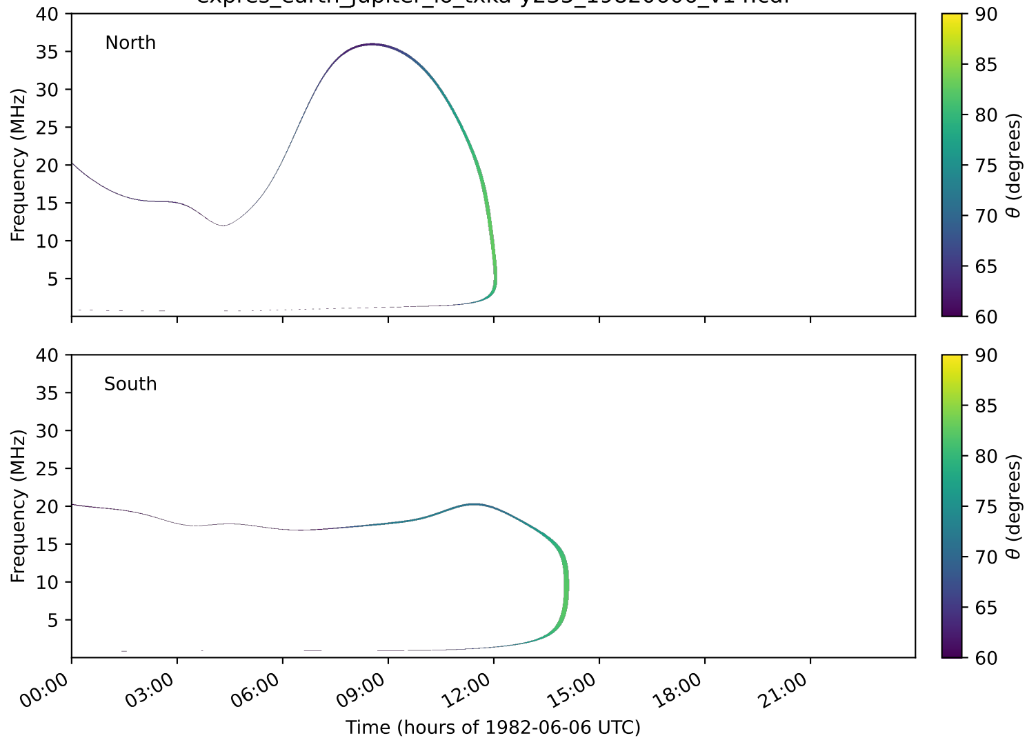
expres_earth_jupiter_io_txka-y235_19820606_v14.cdf
