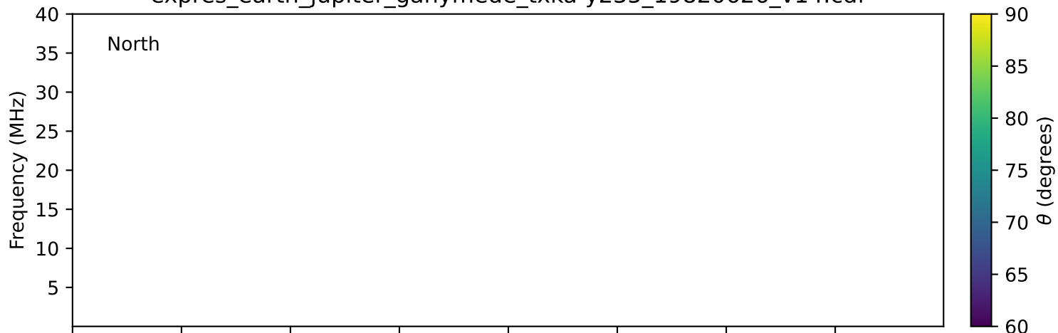
expres_earth_jupiter_ganymede_txka-y235_19820626_v14.cdf
