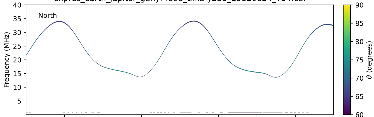
expres_earth_jupiter_ganymede_txka-y235_19820624_v14.cdf
