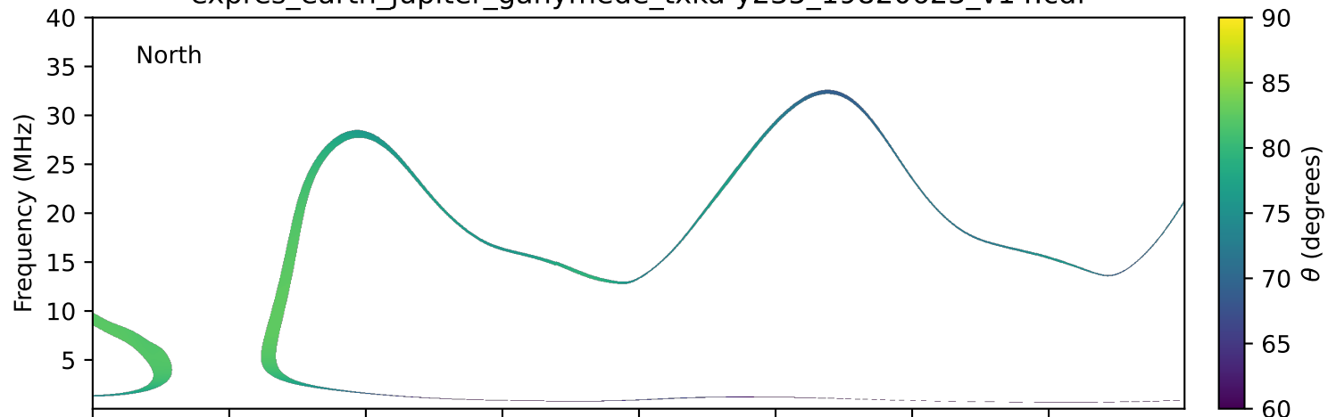
expres_earth_jupiter_ganymede_txka-y235_19820623_v14.cdf
