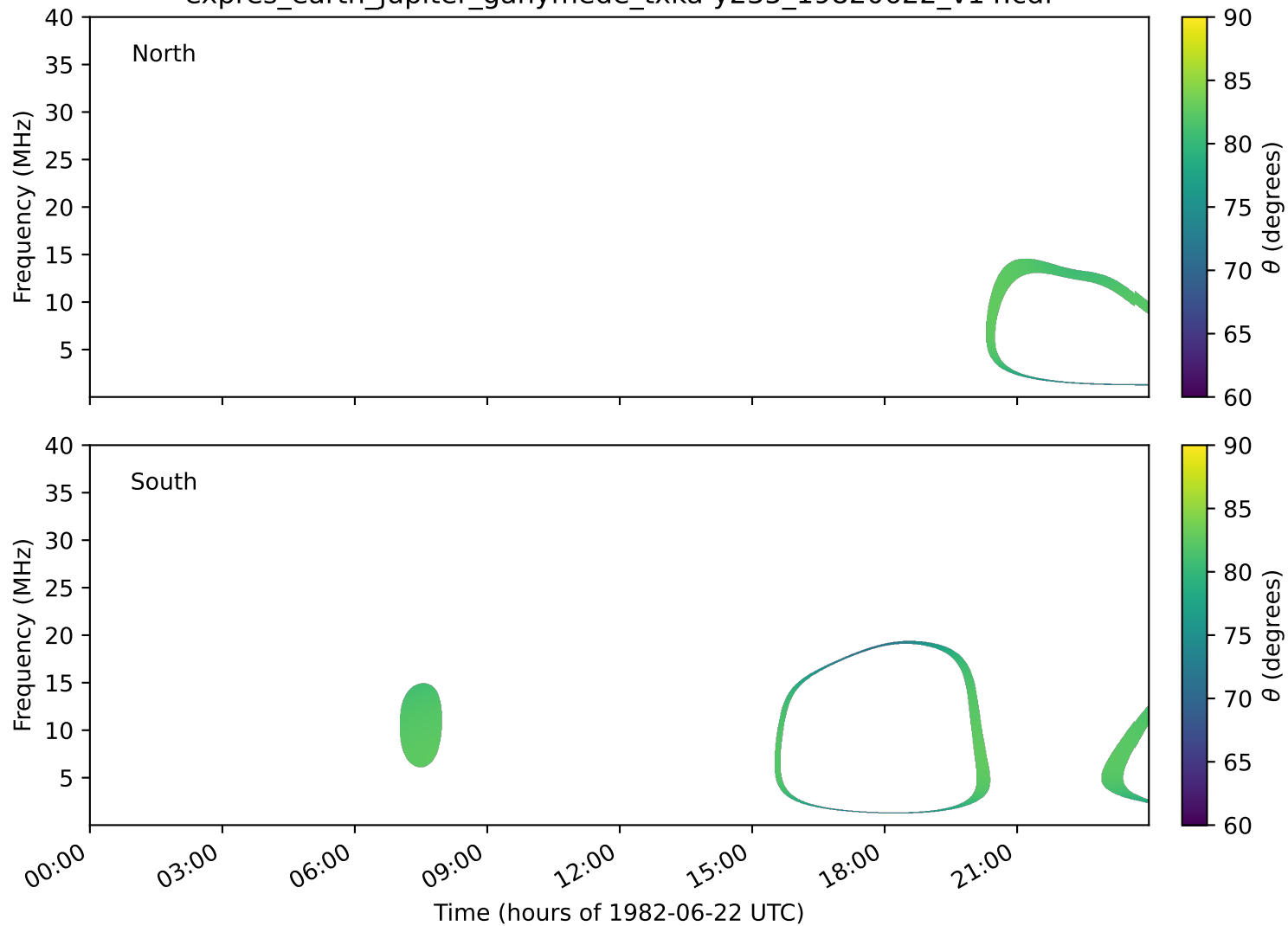
expres_earth_jupiter_ganymede_txka-y235_19820622_v14.cdf
