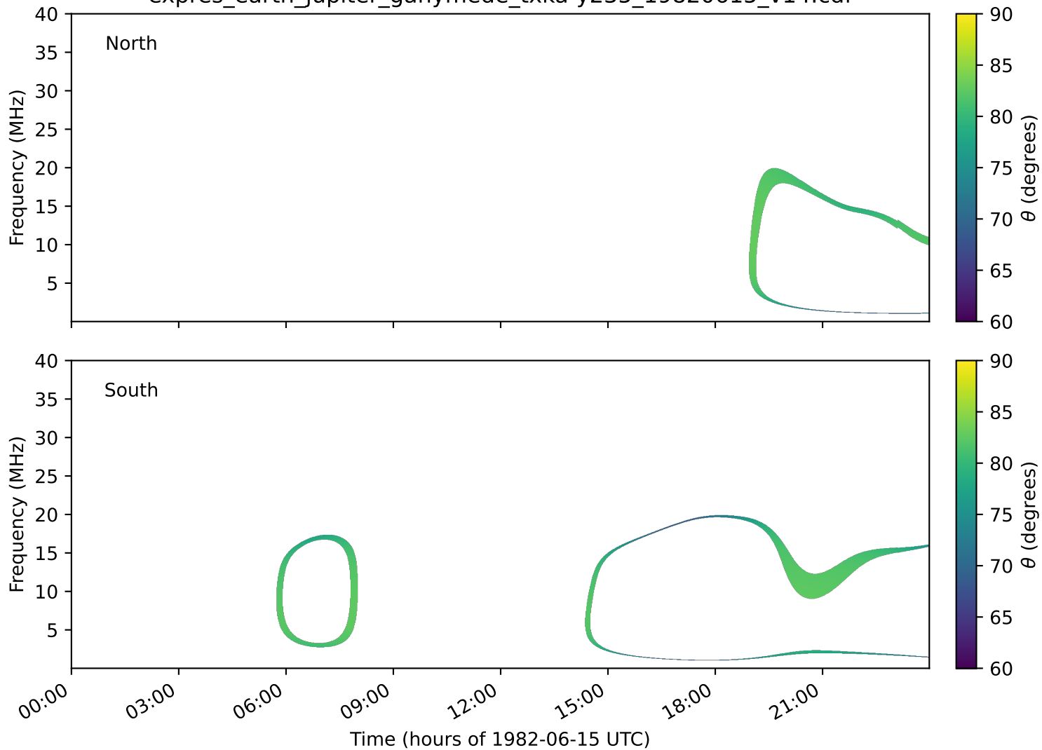
expres_earth_jupiter_ganymede_txka-y235_19820615_v14.cdf
