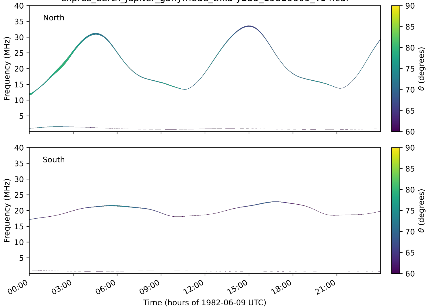
expres_earth_jupiter_ganymede_txka-y235_19820609_v14.cdf
