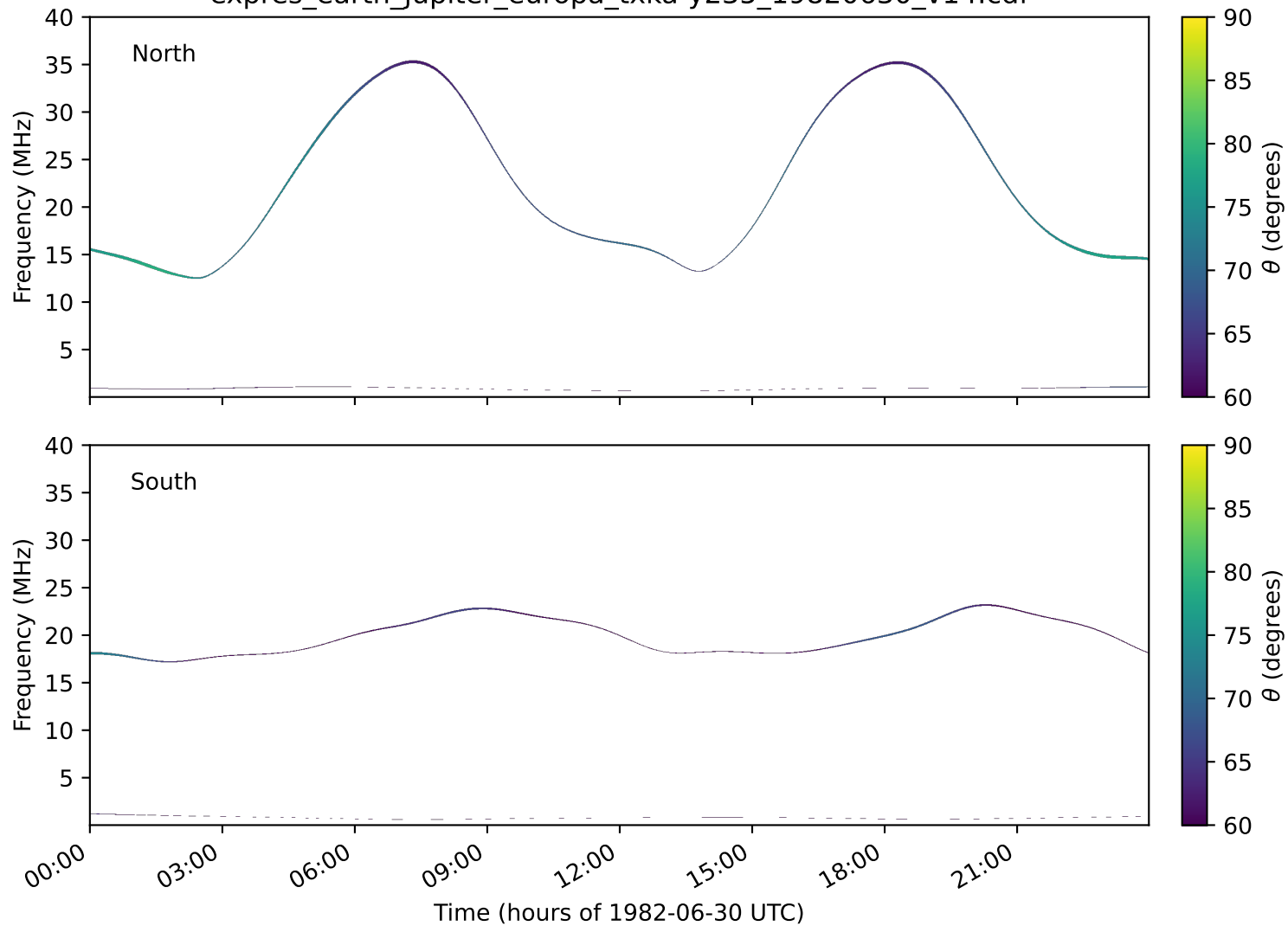
expres_earth_jupiter_europa_txka-y235_19820630_v14.cdf
