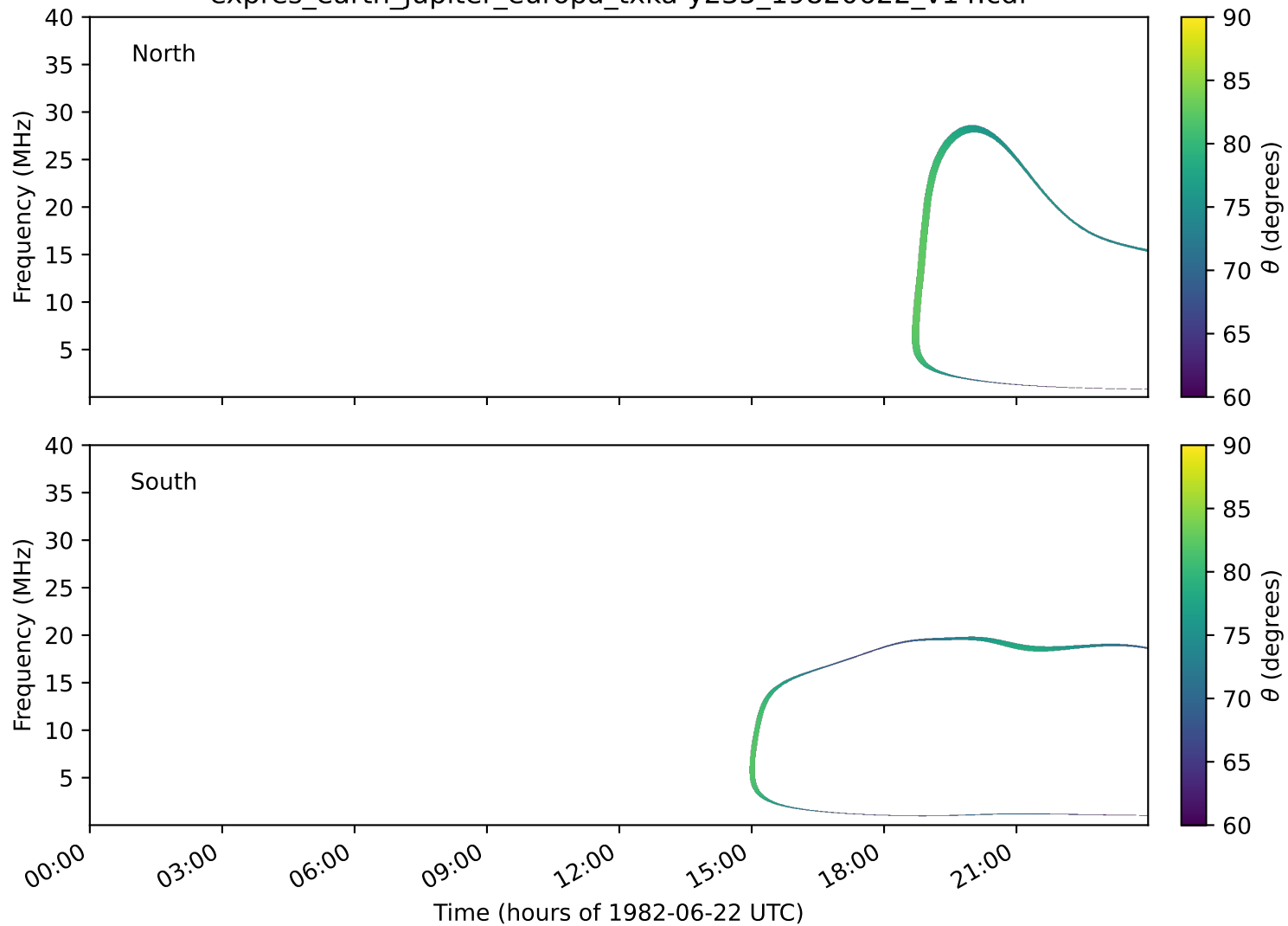
expres_earth_jupiter_europa_txka-y235_19820622_v14.cdf
