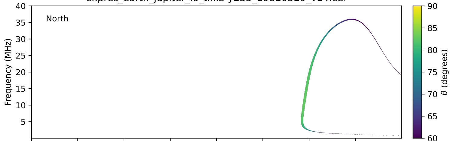
expres_earth_jupiter_io_txka-y235_19820529_v14.cdf
