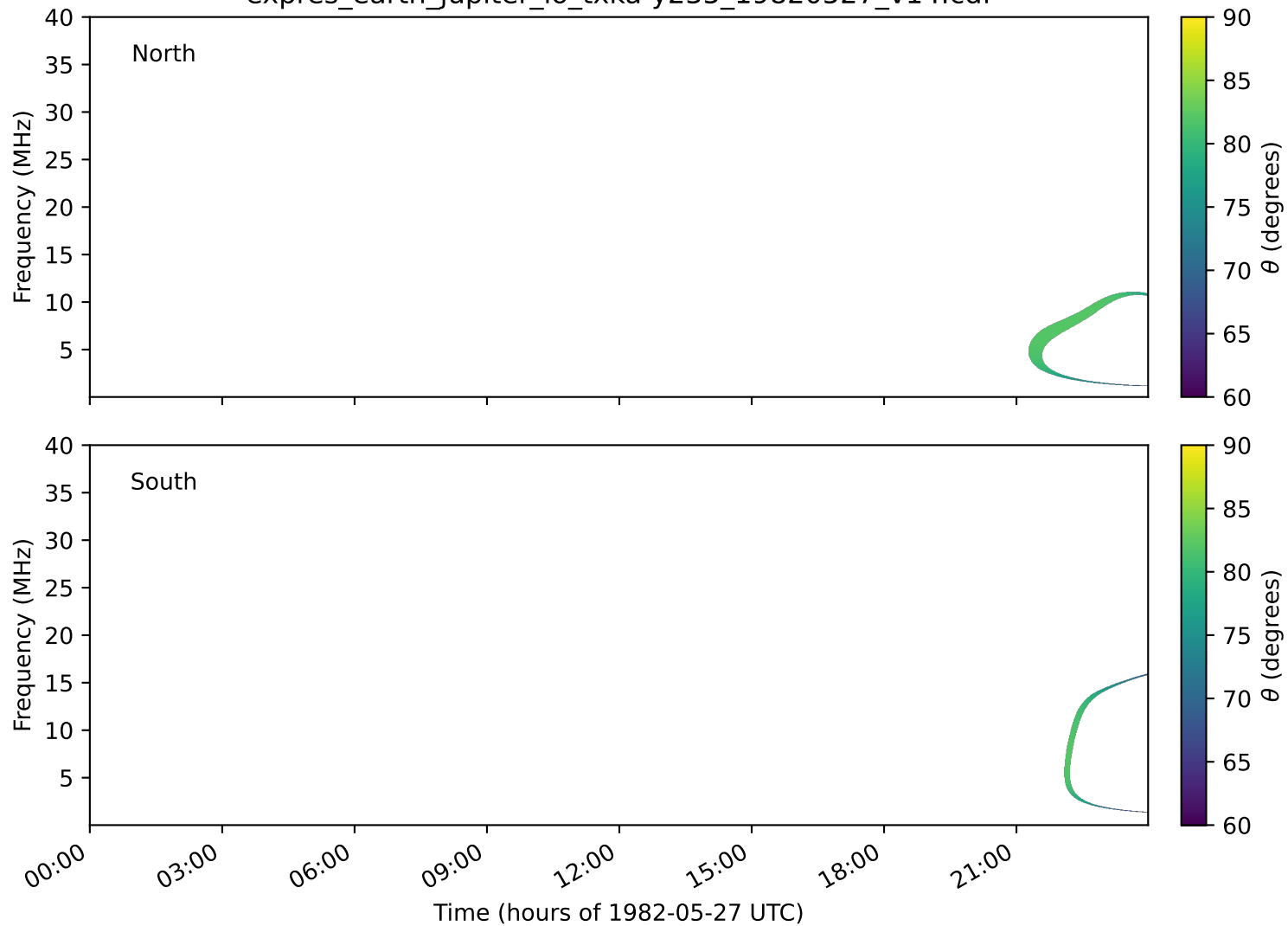
expres_earth_jupiter_io_txka-y235_19820527_v14.cdf
