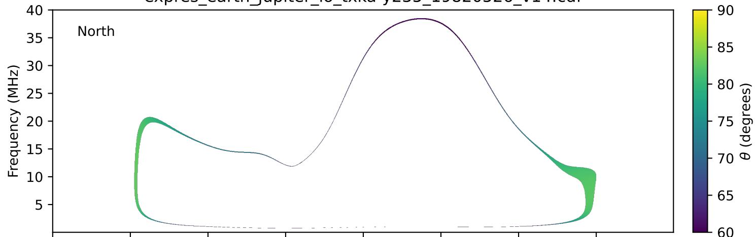
expres_earth_jupiter_io_txka-y235_19820526_v14.cdf
