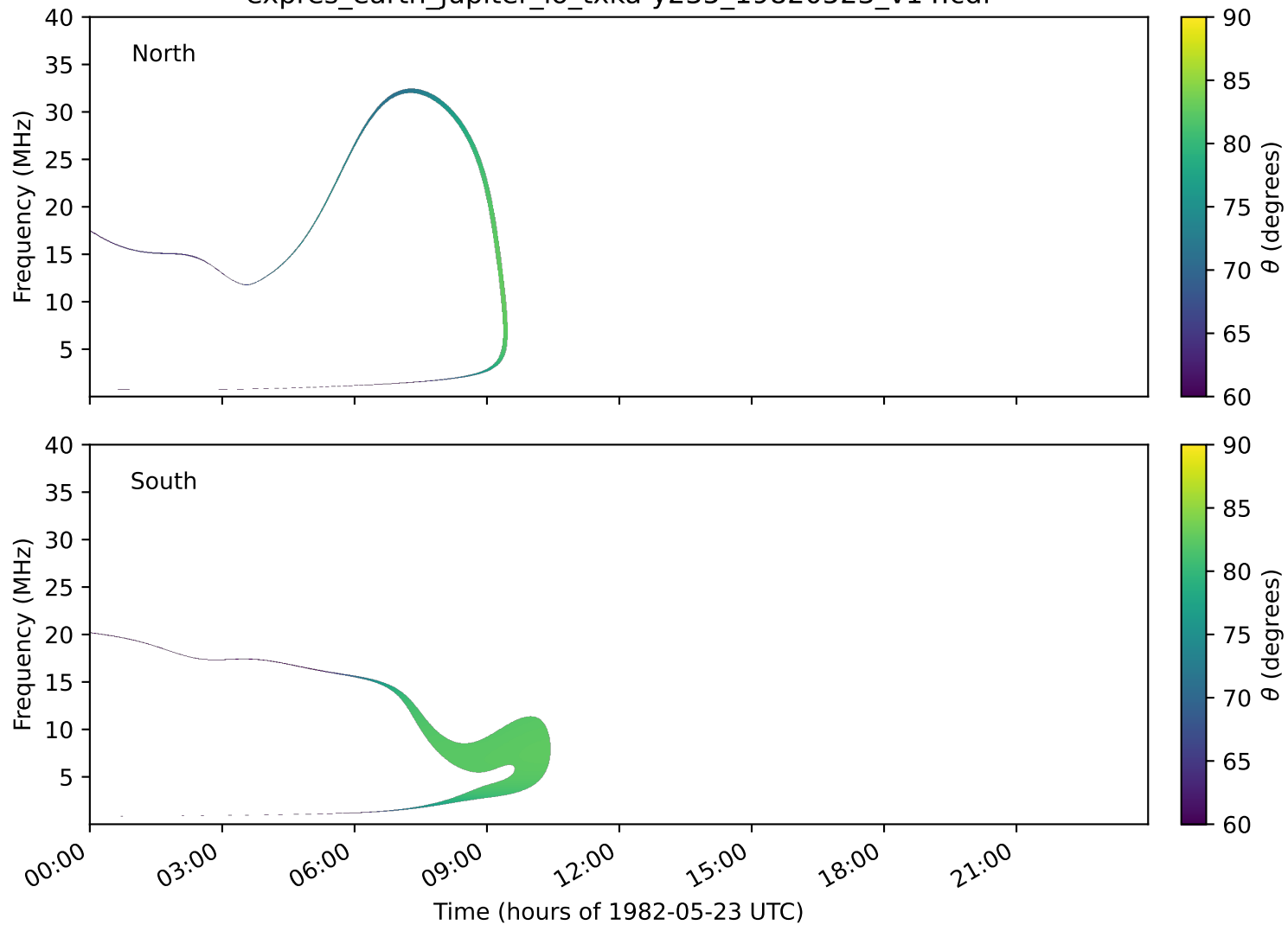
expres_earth_jupiter_io_txka-y235_19820523_v14.cdf
