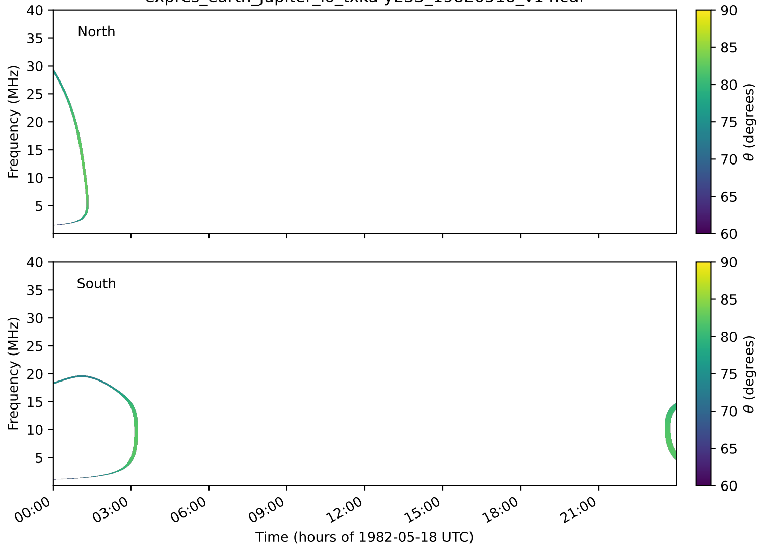
expres_earth_jupiter_io_txka-y235_19820518_v14.cdf
