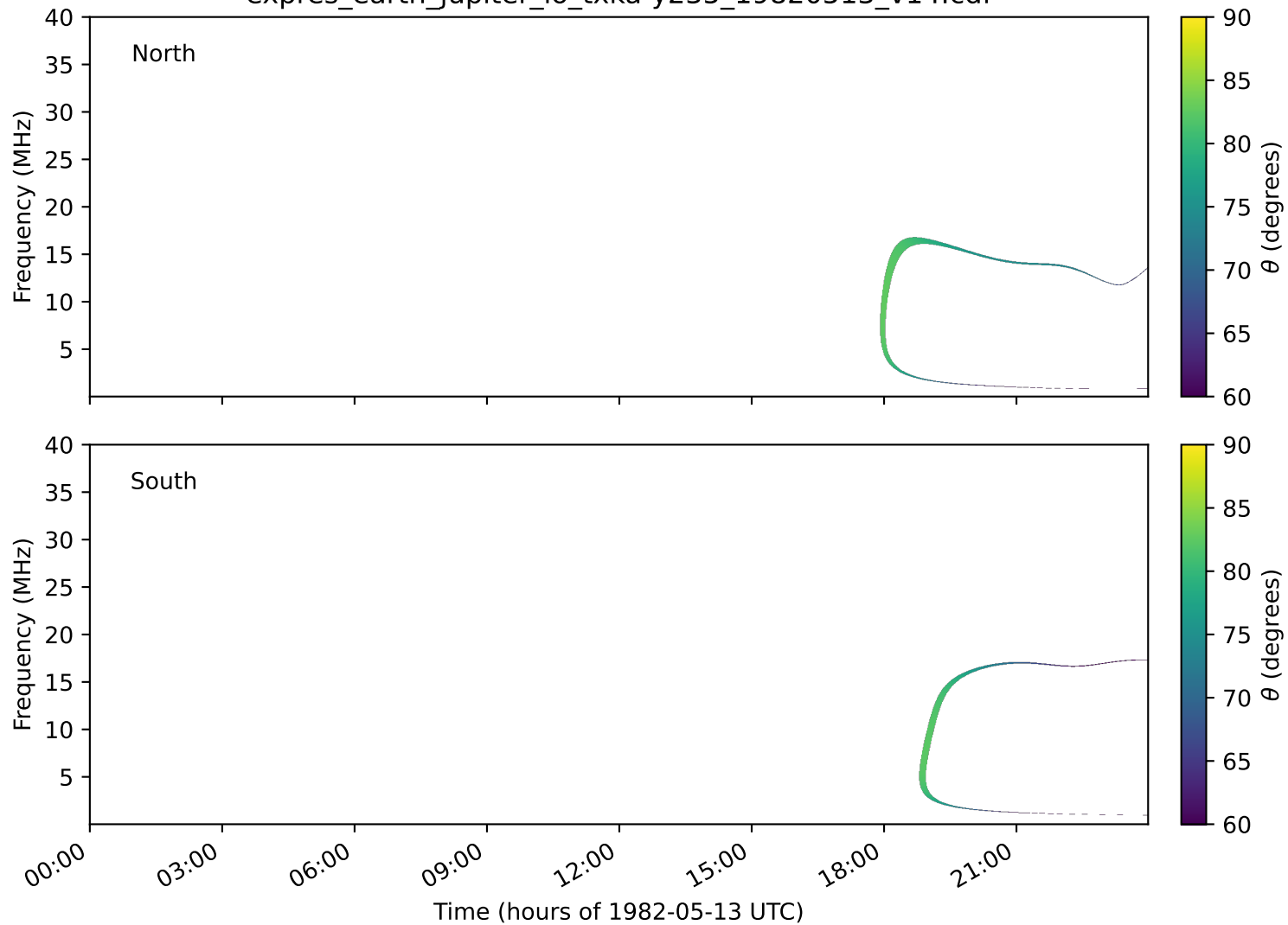
expres_earth_jupiter_io_txka-y235_19820513_v14.cdf
