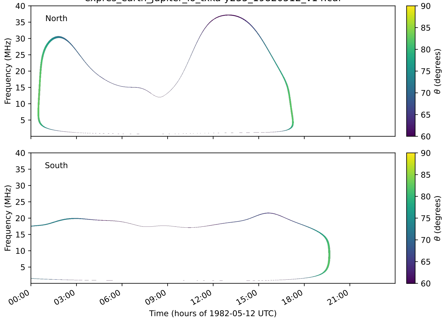
expres_earth_jupiter_io_txka-y235_19820512_v14.cdf
