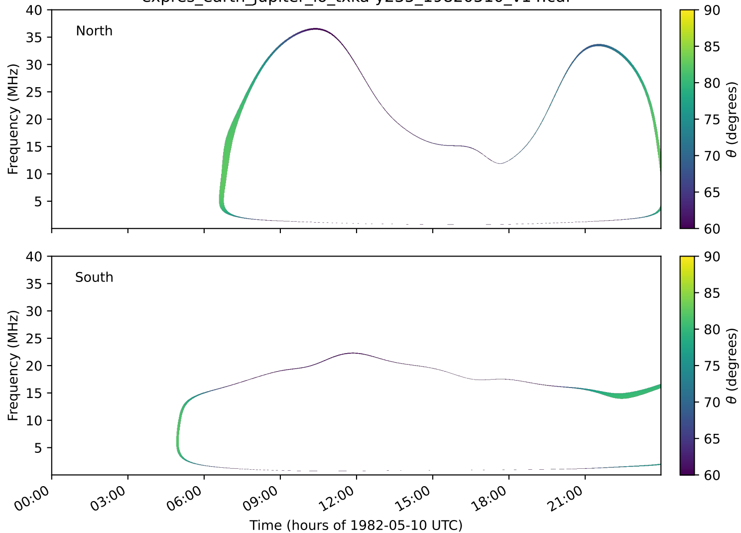
expres_earth_jupiter_io_txka-y235_19820510_v14.cdf
